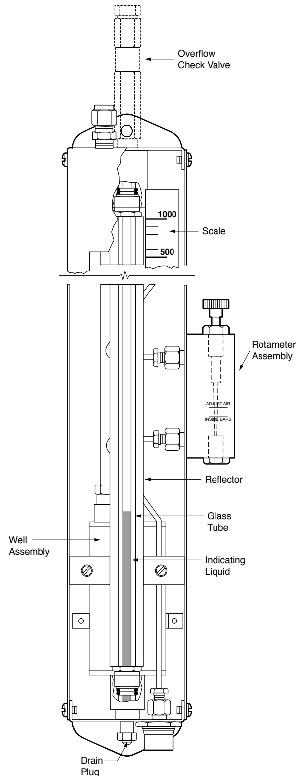
Detail 5993 Internal View
