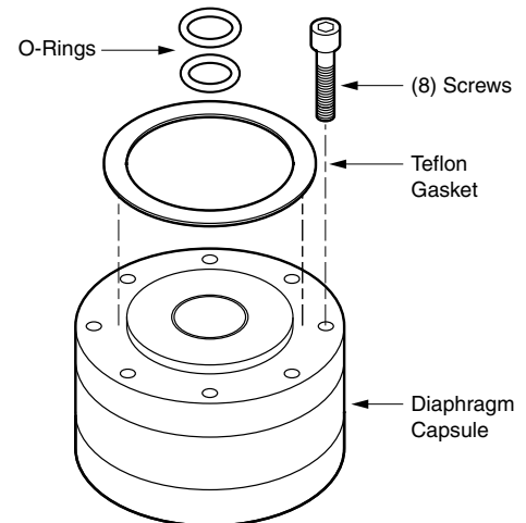
5051-2** Capsule assy. shown
