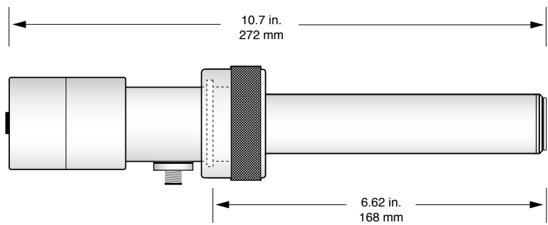
ES2 Slimline Transmitter Model 5502 - Standard Mount
