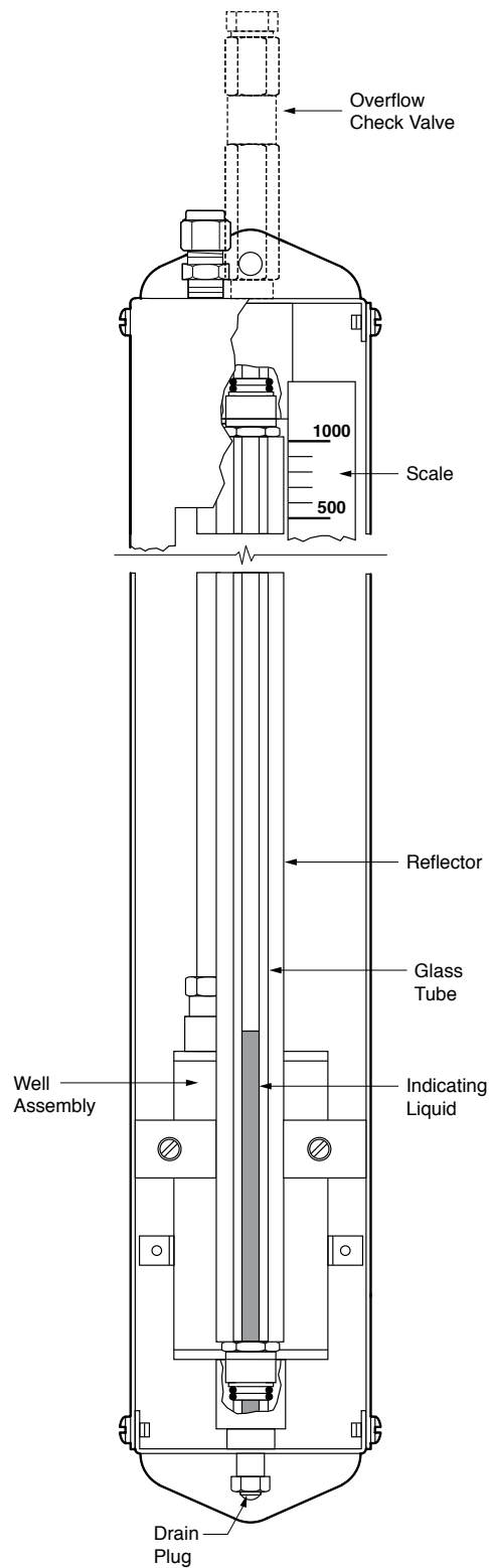
Detail 7750 Internal View
