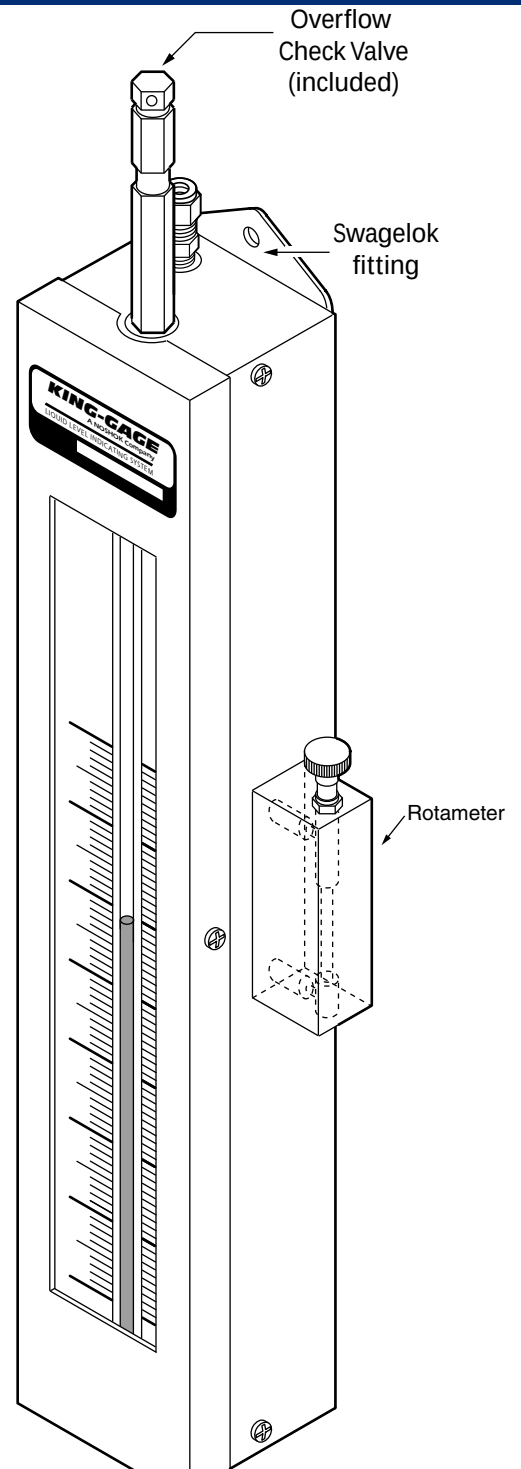
Model 5993 Rotameter Gauge
