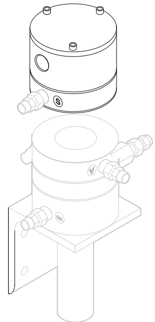
Replacement D/P (transmitter) capsule
