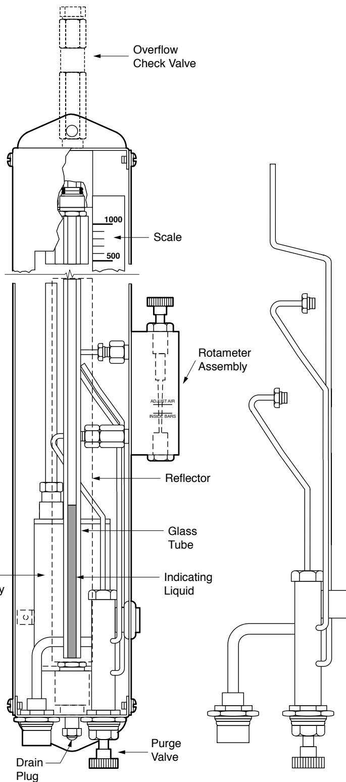
Detail 5990 Internal View
