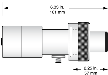
ES2 Slimline Transmitter Model 5501 - Short Mount
