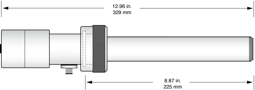
ES2 Slimline Transmitter Model 5503 - Long Mount
